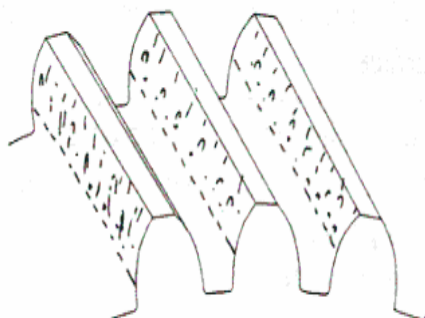
c) Grippage
